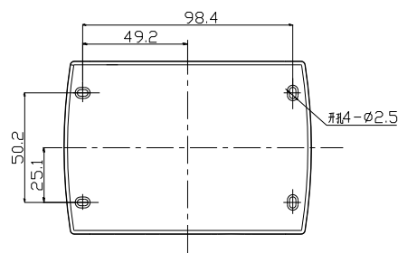
H3N/H4N 墙面安装开孔
